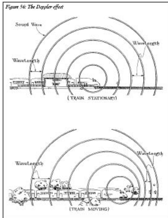
Figure 56: The Doppler effect
