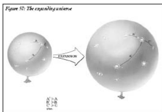
Figure 57: The expanding universe
