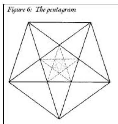
Figure 6: The pentagram
