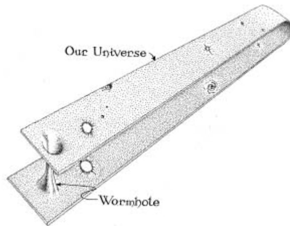
Figure 53: A wormhole
