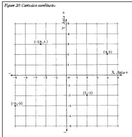
Figure 20: Cartesian coordinates
