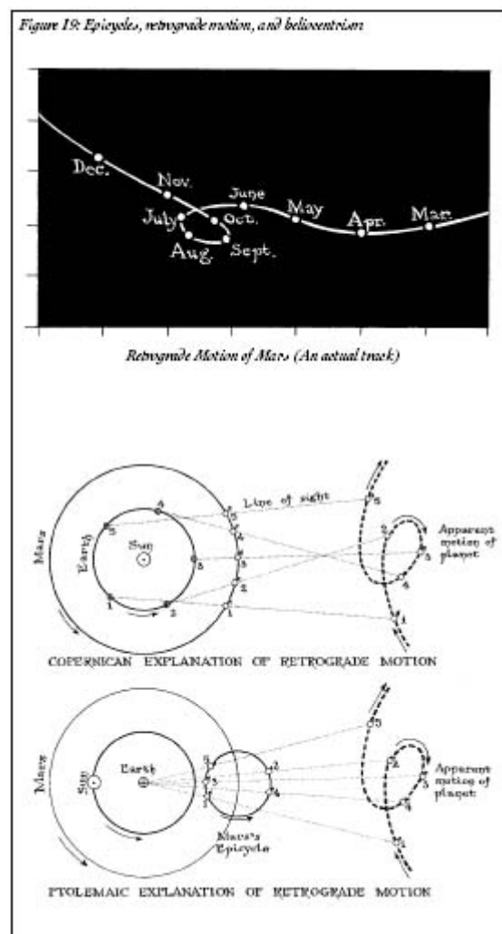
Figure 19: Epicycles, retrograde motion, and heliocentrism
